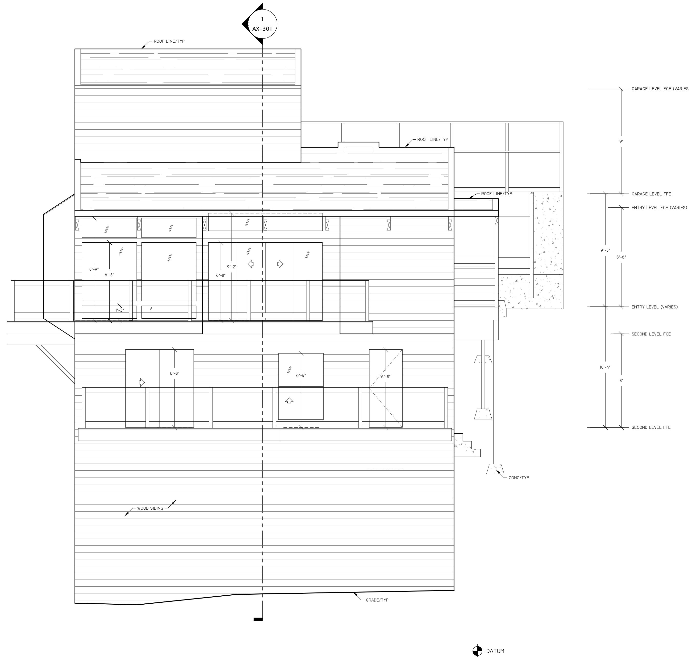
1 EXISTING WEST ELEVATION
