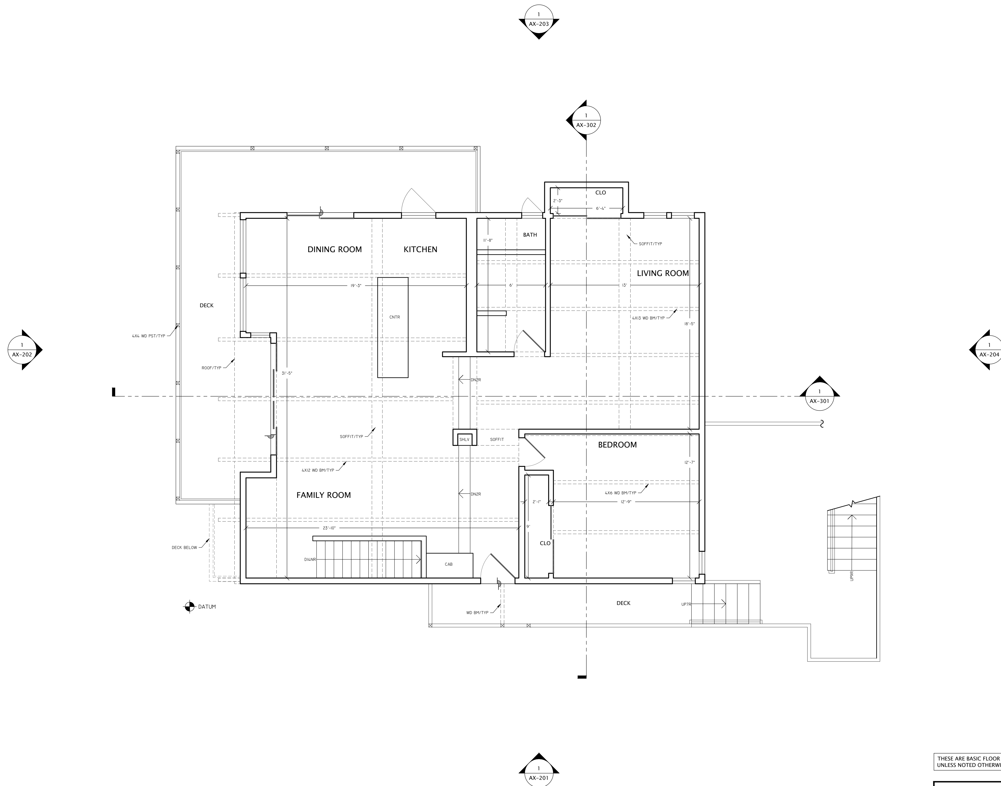
1 EXISTING ENTRY LEVEL FLOOR PLAN 1,304 SQFT GROSS MEASURED AREA 676 SQFT MEASURED EXTERIOR SURFACES
