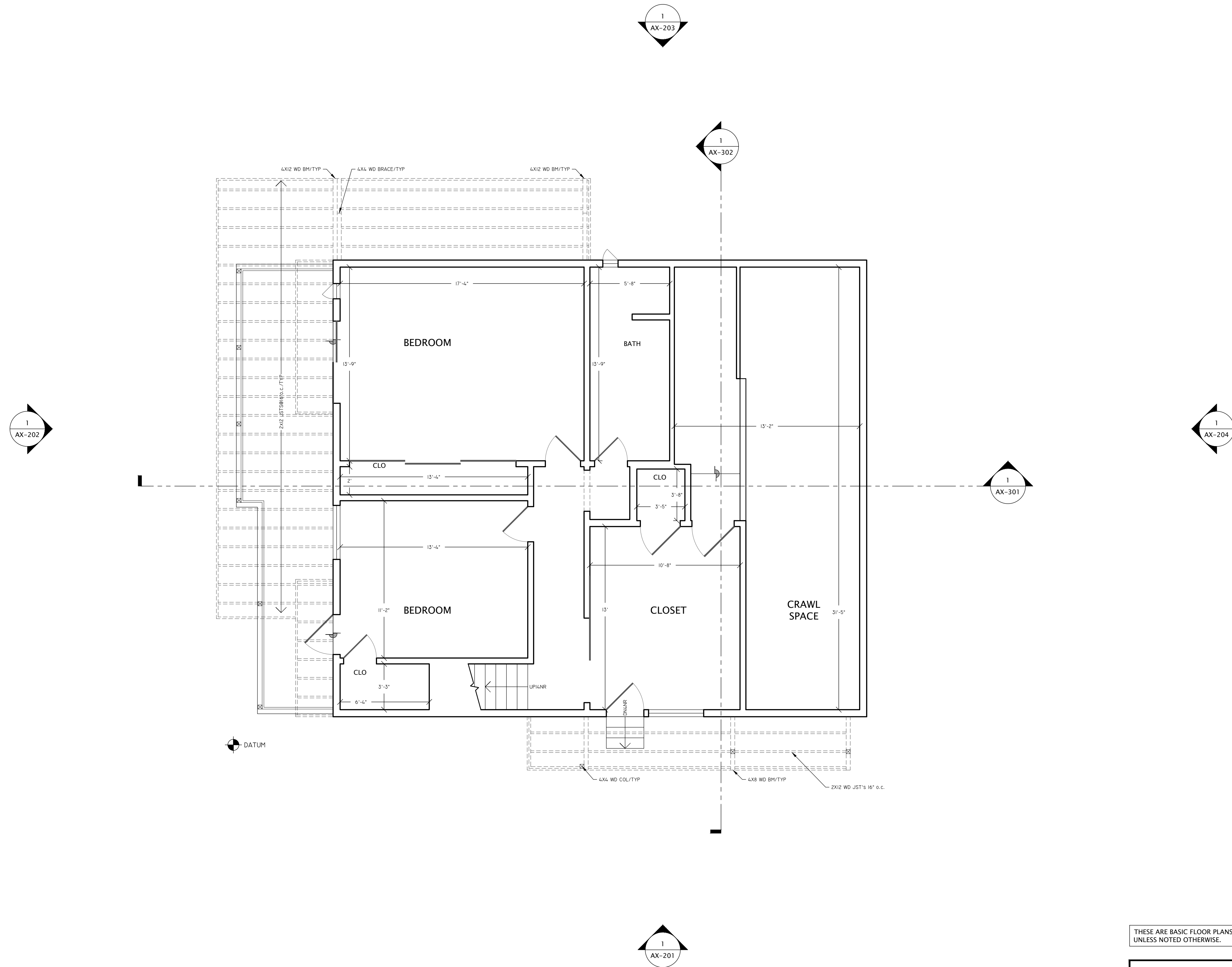
1 EXISTING SECOND LEVEL FLOOR PLAN 1,229 SQFT GROSS MEASURED AREA 203 SQFT MEASURED EXTERIOR SURFACES
