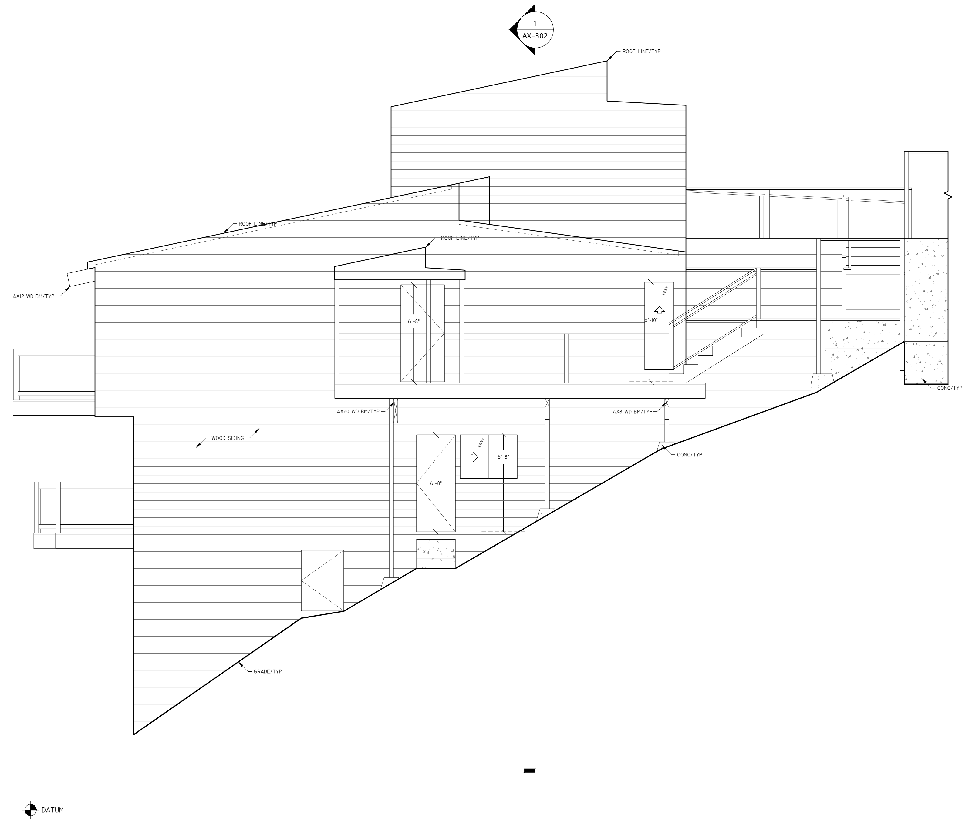
1 EXISTING SOUTH ELEVATION
